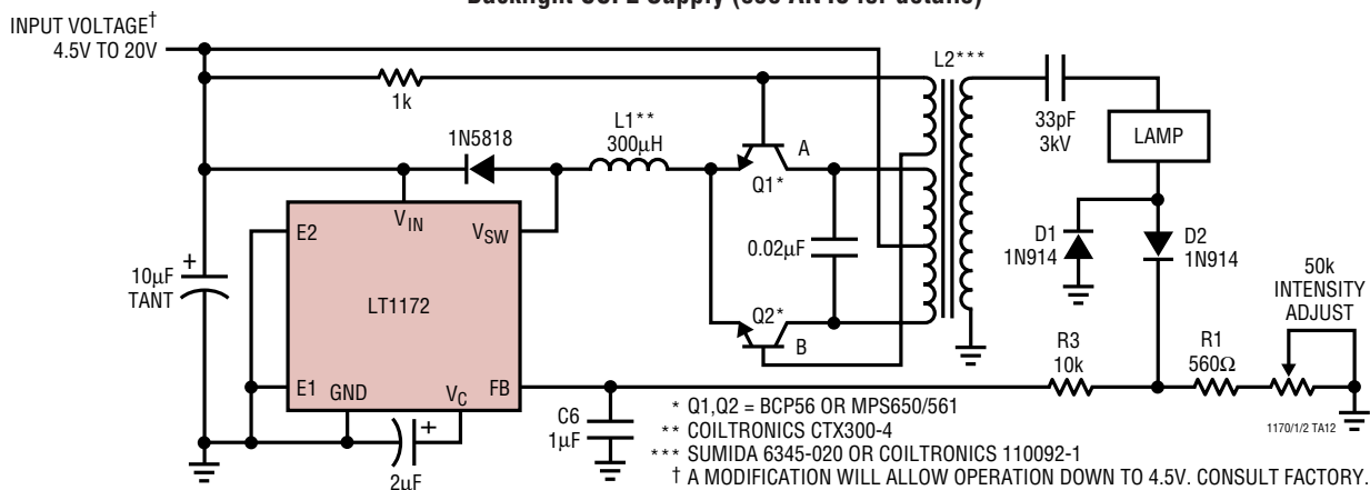
Backlight CCFL Supply (see AN45 for details)
