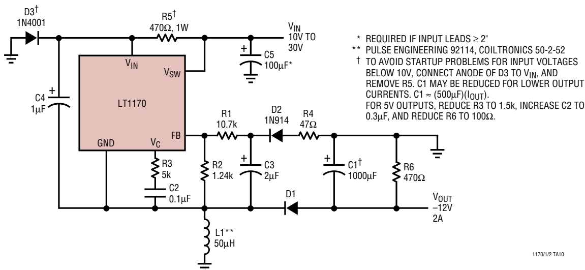
High Efficiency Constant Current Charger
